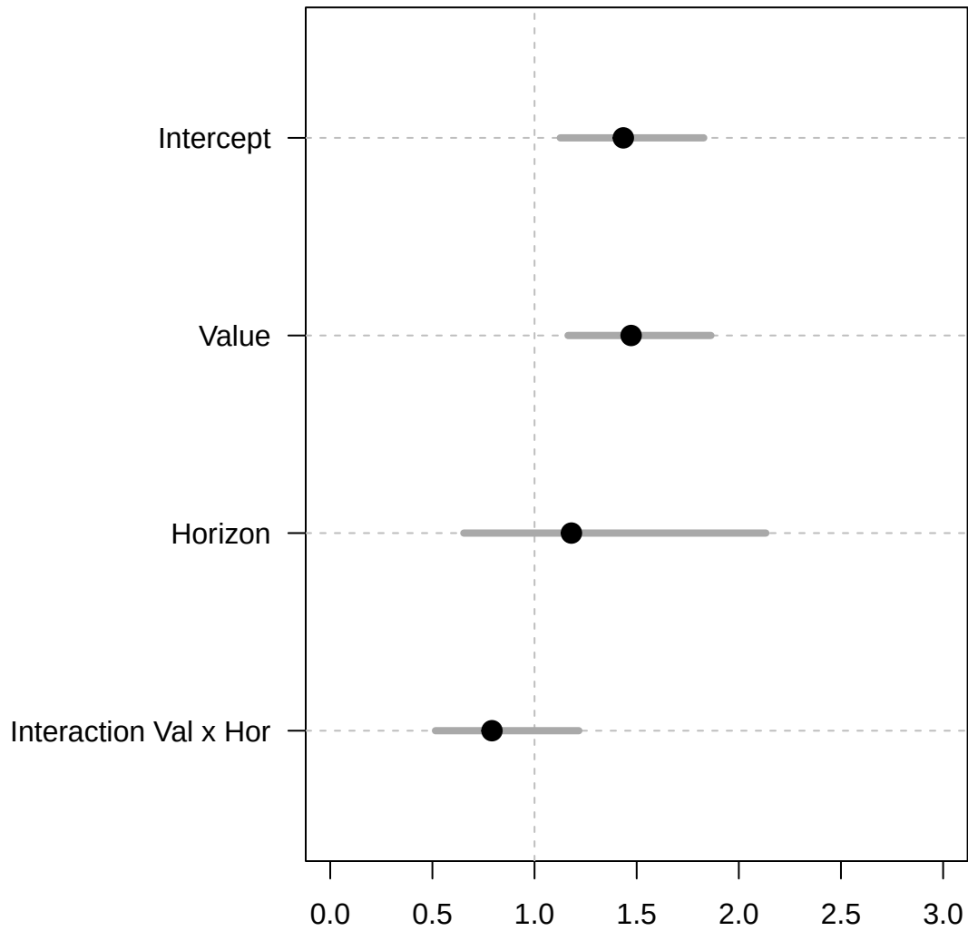
Odds ratio fits from Bayesian model
