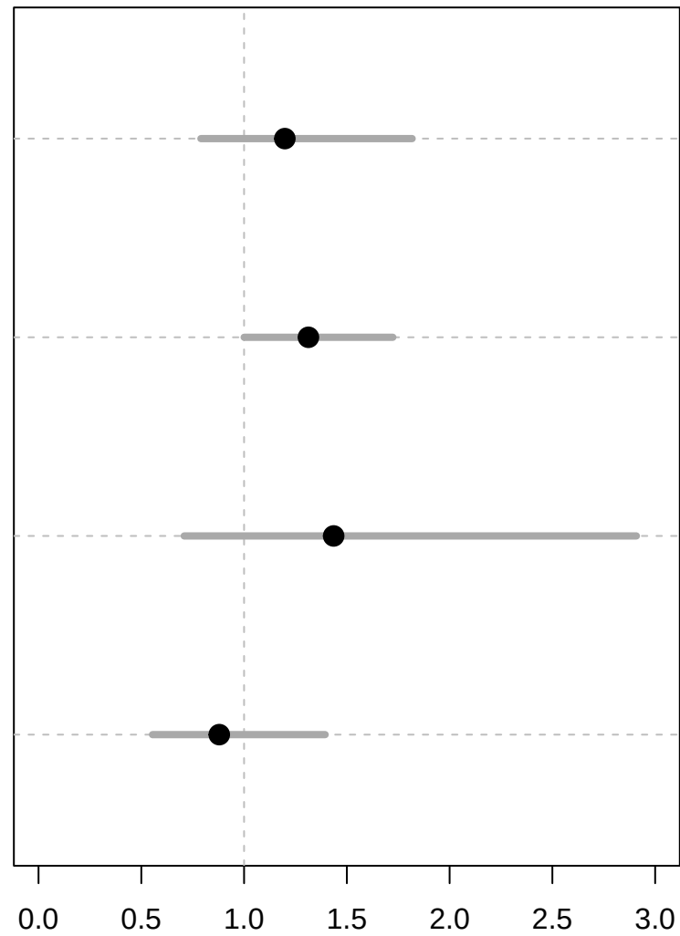
Odds ratio fits from GLM
